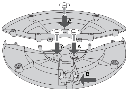
Figure 2 Assembling the foot
